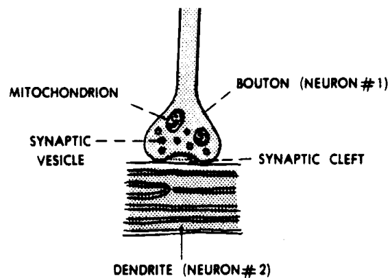
Figure 5-2. A synapse.
